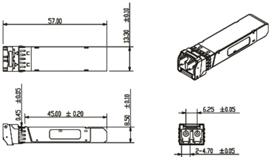
Figure4. Mechanical Specifications
