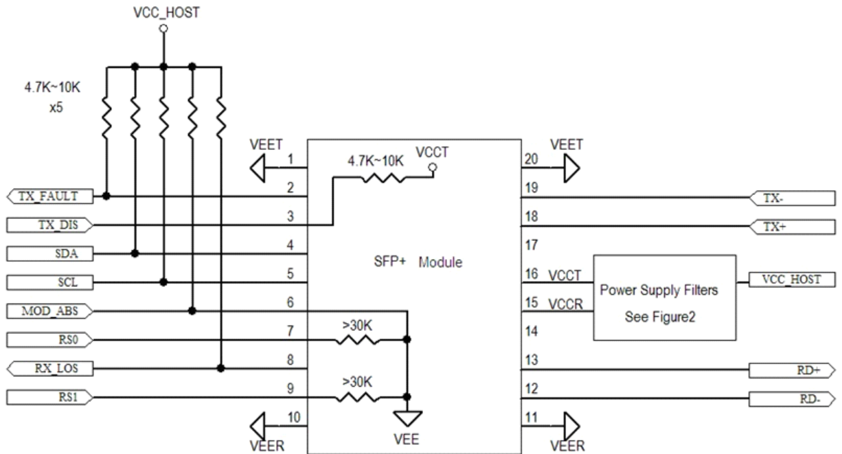
Figure3. Host-Module Interface
