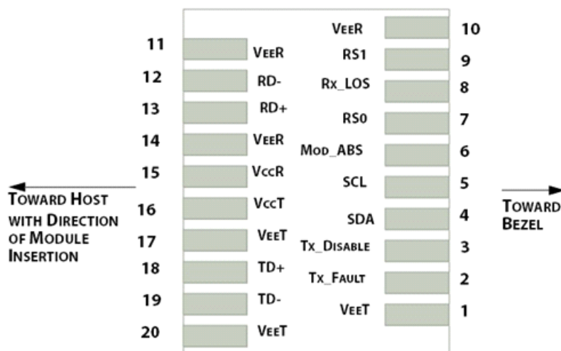
Figure1.Electrical Pin-out Details
