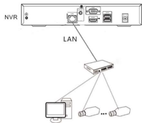
Figure 4.3 Topology of a Network
